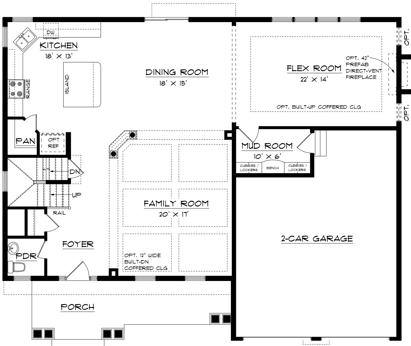
FIRST FLOOR PLAN ROOM DIMENSIONS APPROXIMATE
